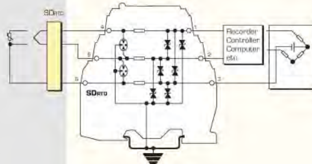
3-wire RTDs
