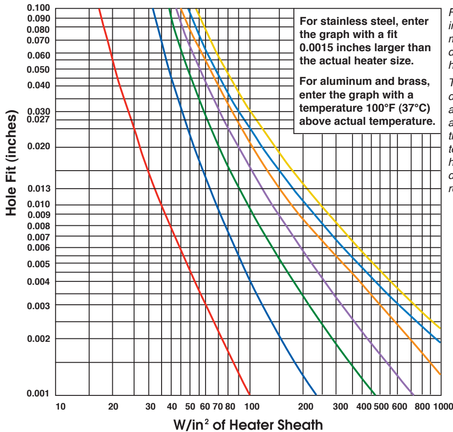
Graph D: Recommended Maximum Hole Fit For Heating Metals
