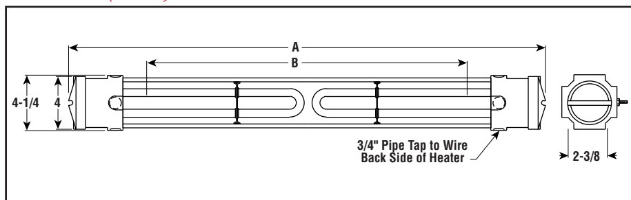
Dimensions (Inches)
