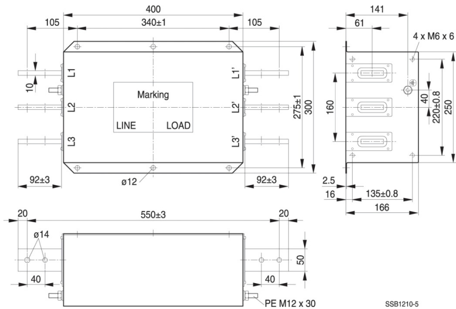
(1600 A) KRF1600VCB
