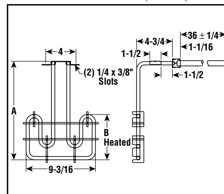
PTHT — Dimensions (Inches)
