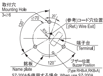
取付面寸法図 Installation Dimensions
