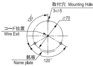
取付面寸法図 Installation Dimensions
