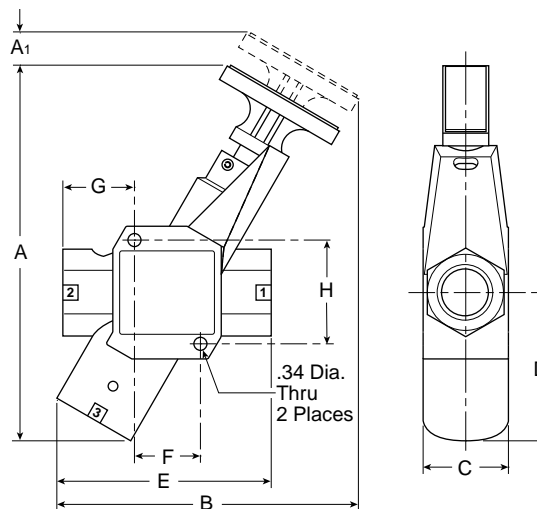
LV Series, 3/4" Exhaust Port Inches (mm)
