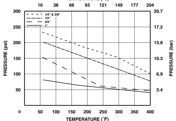
PARFLARE FITTINGS WITH HT NUT ASSEMBLIES PRESSURE VS. TEMPERATURE
