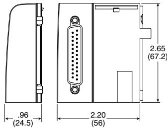
20-Pin, Multi-Connector
