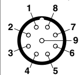
M23 Female
