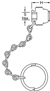
CGA Plug 510, 580 & 590
