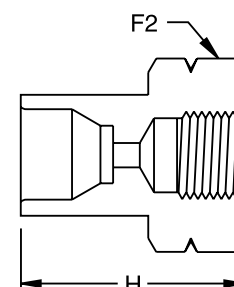
NPT Female CGA 350
