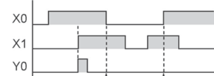
[Time chart 1]
