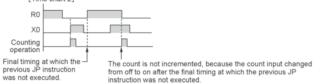
[Time chart 2]
