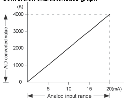
Conversion characteristics graph
