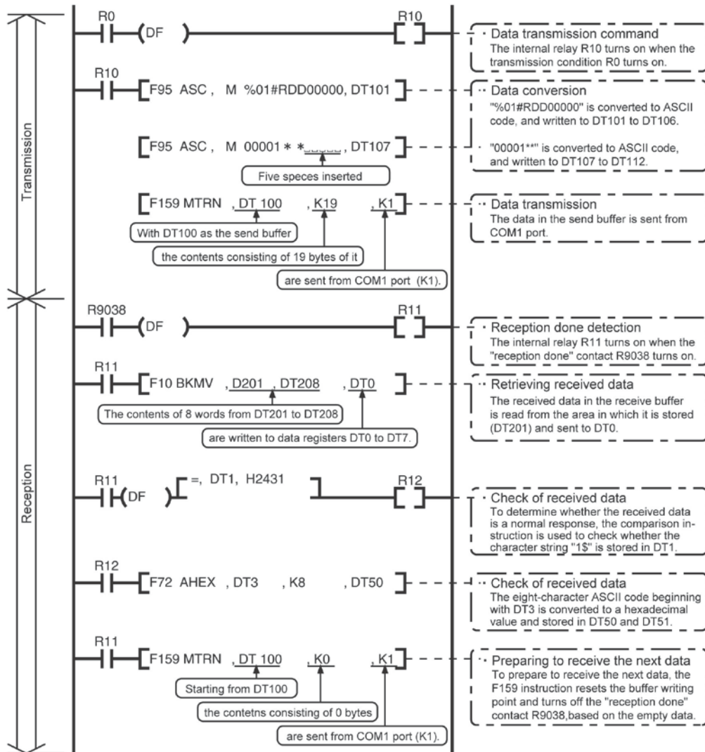
Send buffer
