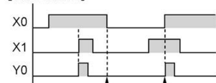
[Time chart 2]
