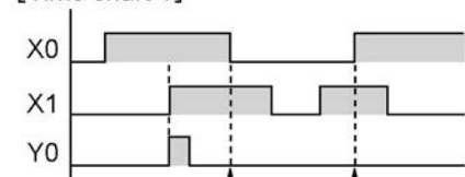
[Time chart 1]
