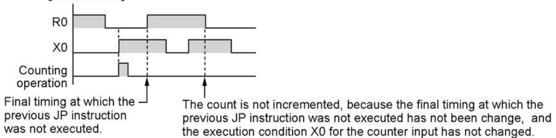
[Time chart 2]
