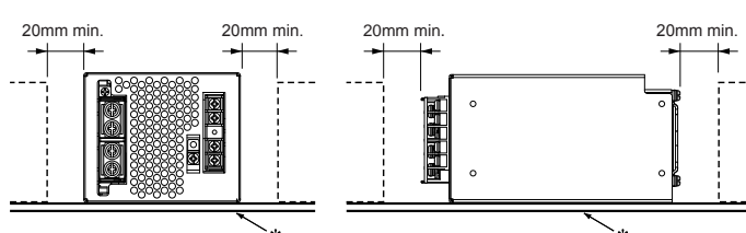
Bottom-mounting
