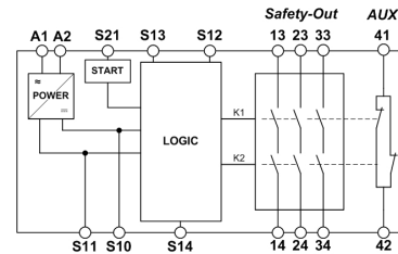
Fig. 1 Block diagram SR103AM
