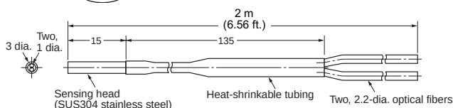
E32-D12 (Free-cut)
