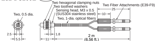
E32-DC200E (Free-cut)
