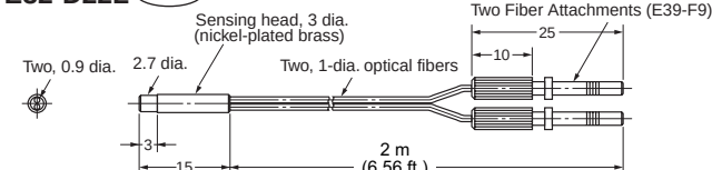
E32-D22L (Free-cut)
