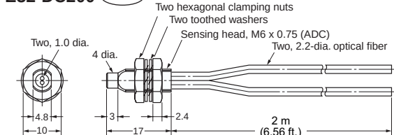
E32-DC200 (Free-cut)
