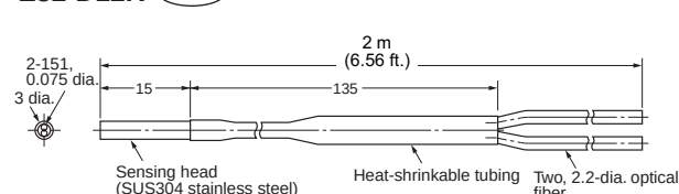
E32-D12R (Free-cut)
