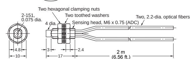
E32-D11R (Free-cut)
