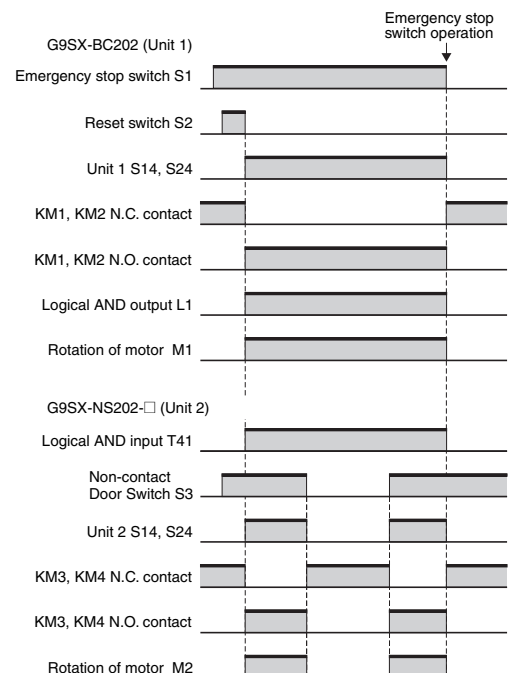
Timing chart
