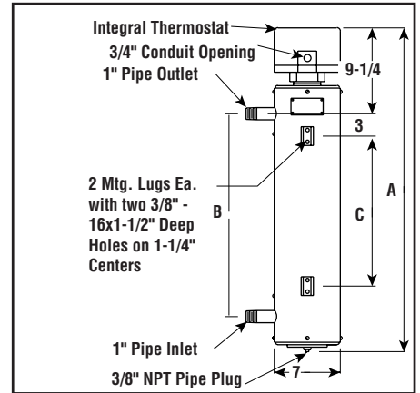
Dimensions (Inches)
