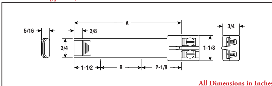
Dimensions (type NS)
