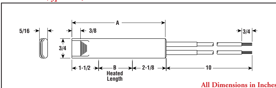
Dimensions (type NSL)
