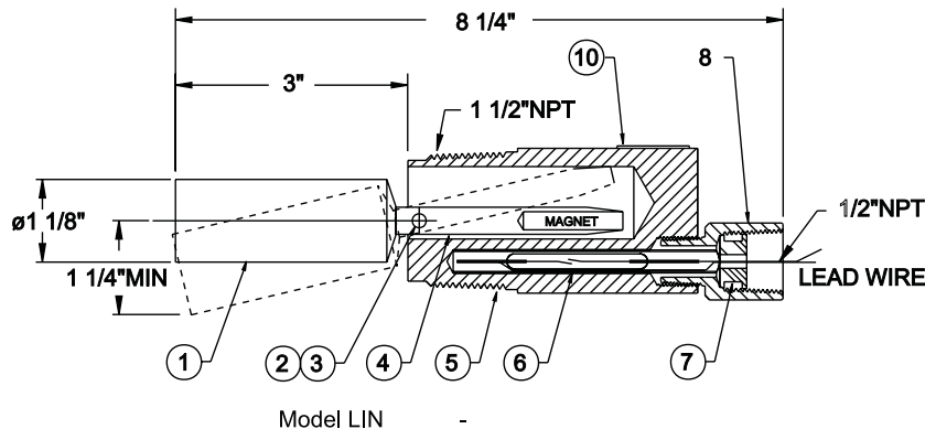
Figure 2, LINC L471-02 & 03 Level Switch
