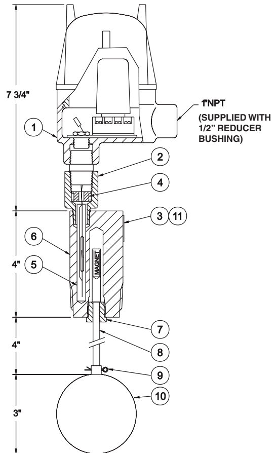
Model LINC-LV471-04-04-N Normally Closed
