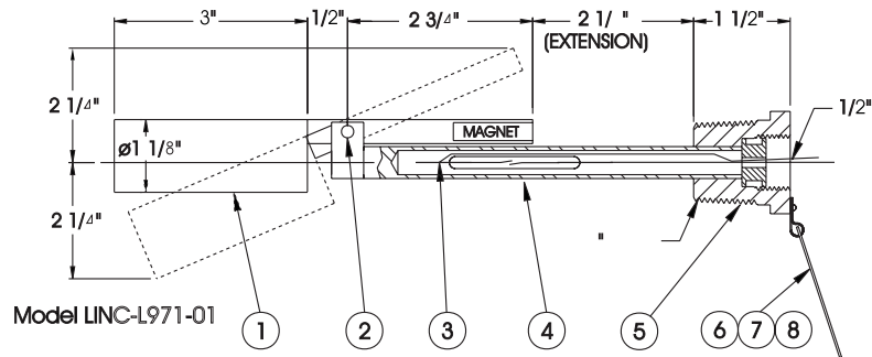
Figure 10, LINC L971-01 and L971-01-04-N Series: Extended Body
