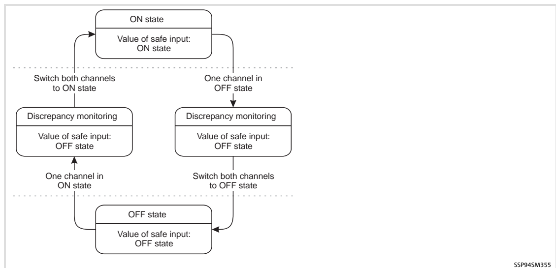
Fig. 1-5 Status behaviour - contact function test
