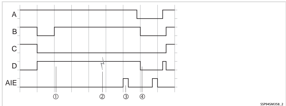
Fig. 1-7 Contact function test - faulty input signals
