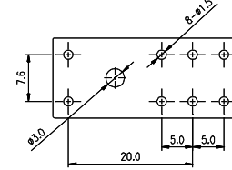
SQ2V-63 PCB pin layout
