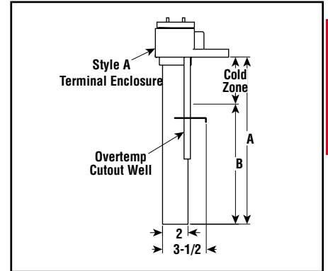
Dimensions (Inches)
