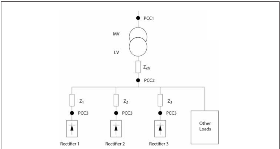
Fig. 7.4 Example of Distribution System
