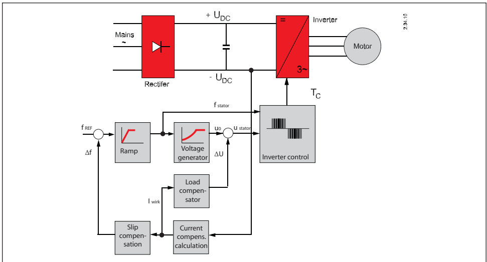
Fig. 2.22 Structure Scalar type Frequency Converter with compensation
