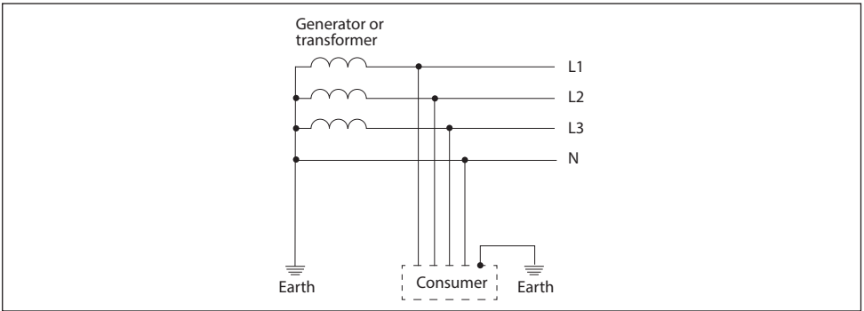
Fig. 6.4 TT system: Earthed neutral conductor and individual equipment/installation earthing
