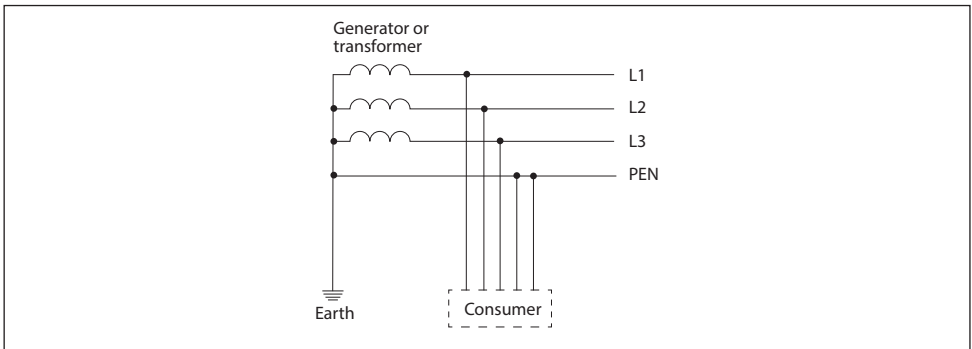
Fig. 6.2 TN-C system: In the entire system, the neutral conductor and the PE conductor are combined in the PEN conductor.
