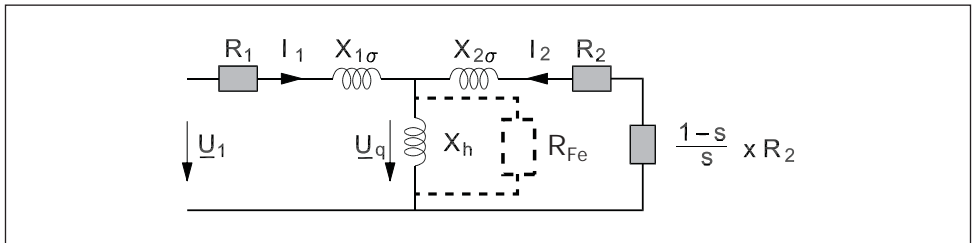
Fig. 1.15 Equivalent circuit diagram (one phase) for a motor operating under load
