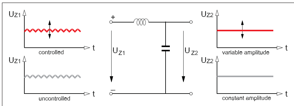
Fig. 2.11 Constant DC intermediate circuit
