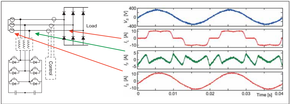
Fig. 7.6 Operation Principle of an Active Filter
