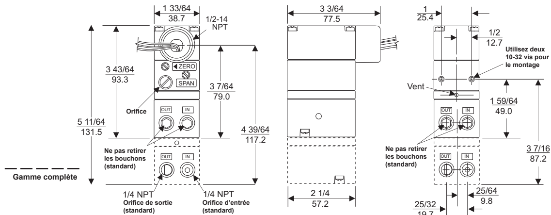
Figure 1. Dimensions TA6000
