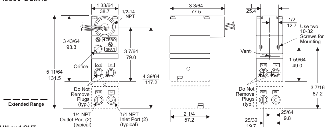
Figure 1. TA6000 Outline Dimensions
