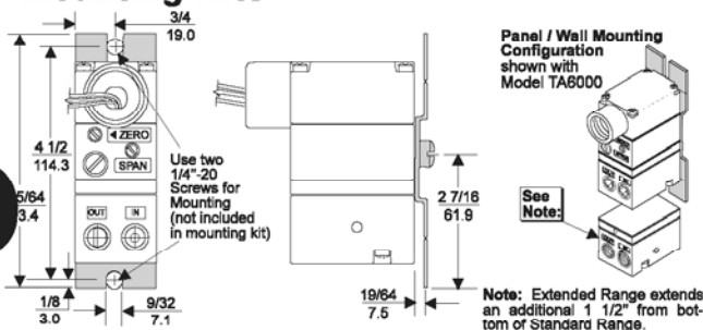
Mounting Bracket: 16799-1
