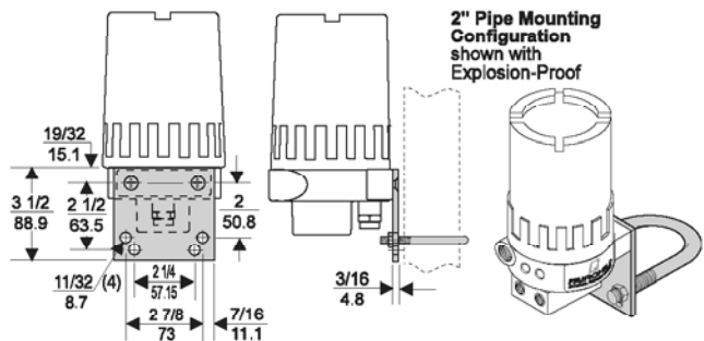
Mounting Bracket: 18187-1
