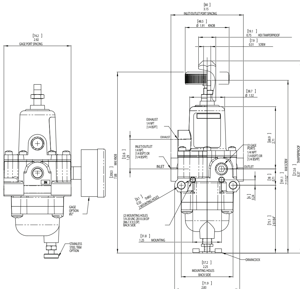
Figure 1. Model 65 Outline Dimensions
