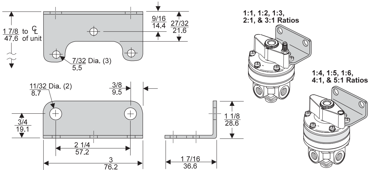
Figure 2. Mounting Bracket 09921. (Sold Separately)
