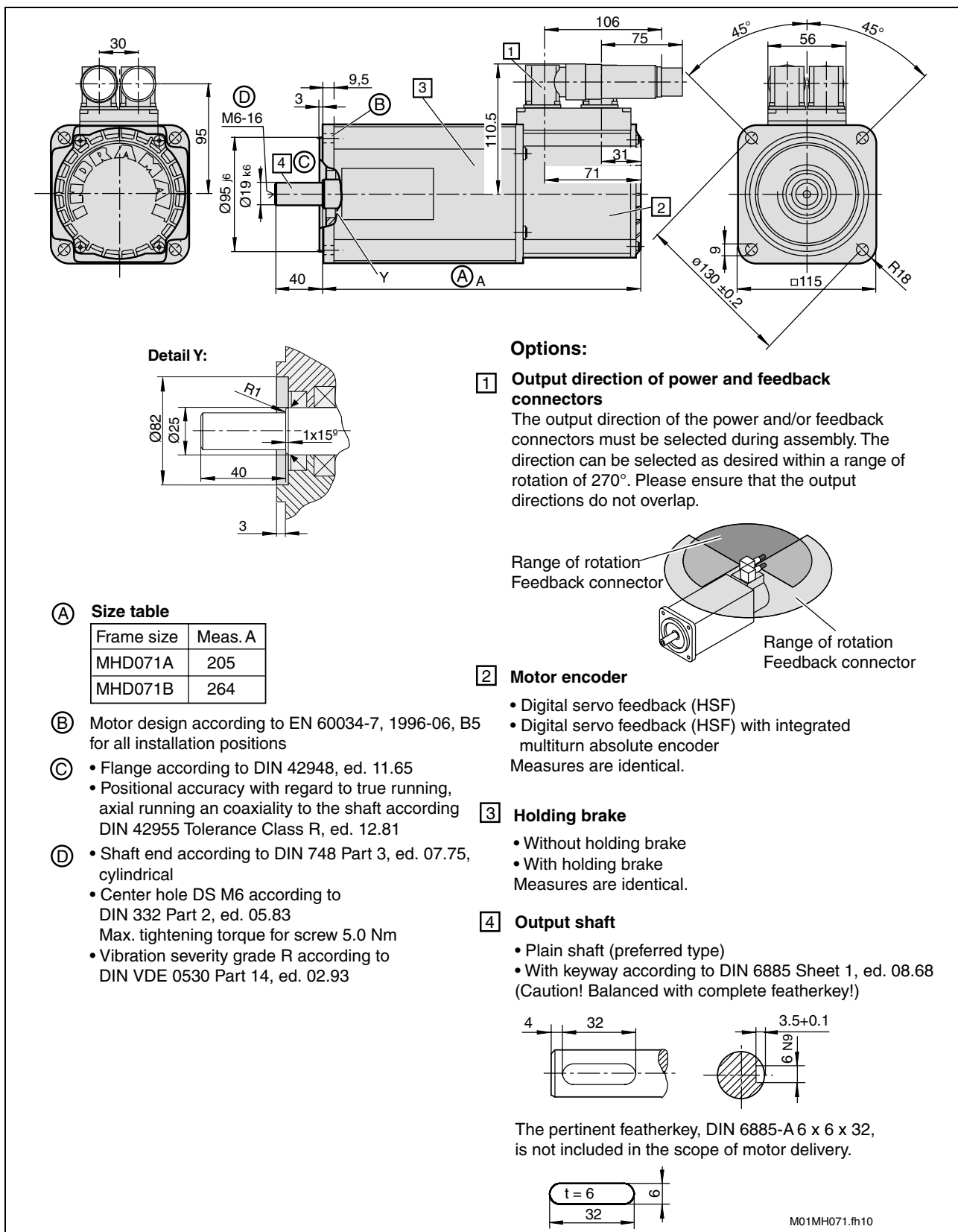
Fig. 7-9: Dimensional details of MHD071
