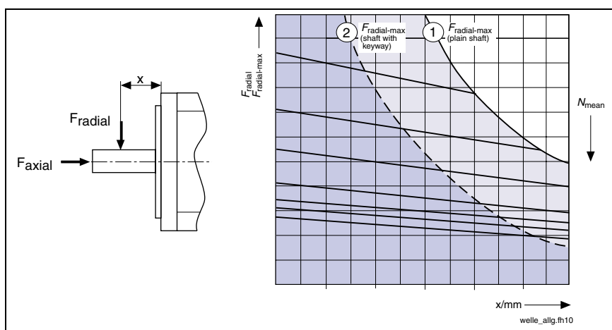
Fig. 16-22: Example of a shaft load diagram
