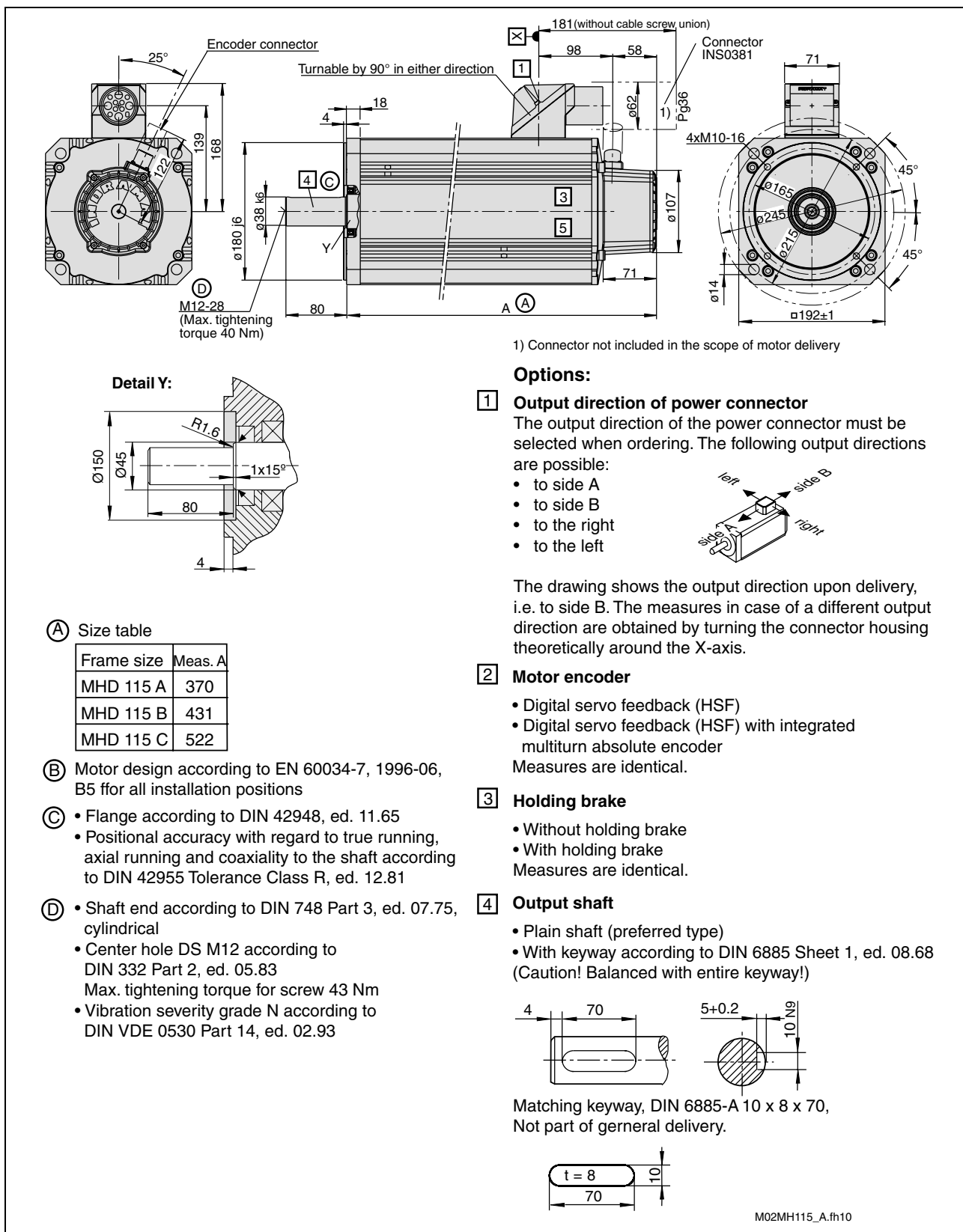
Fig. 12-17: Dimensional details of MHD115.-...-A
