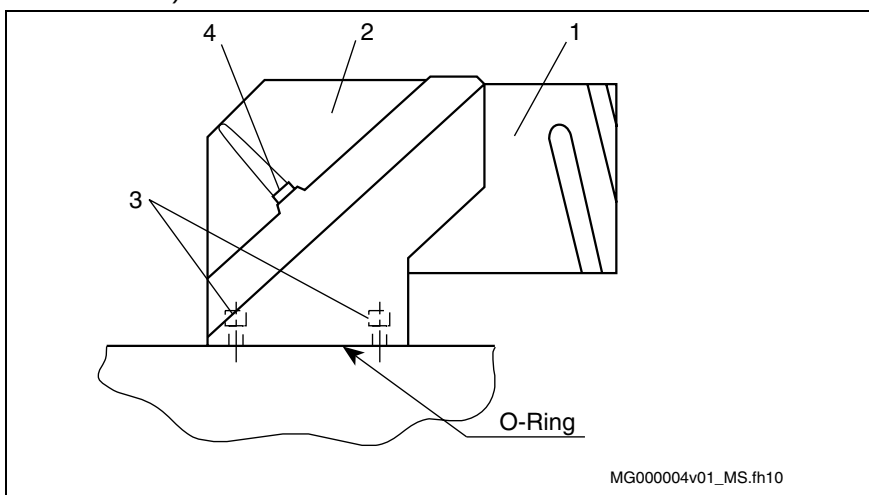
Fig. 18-2: Power connector
