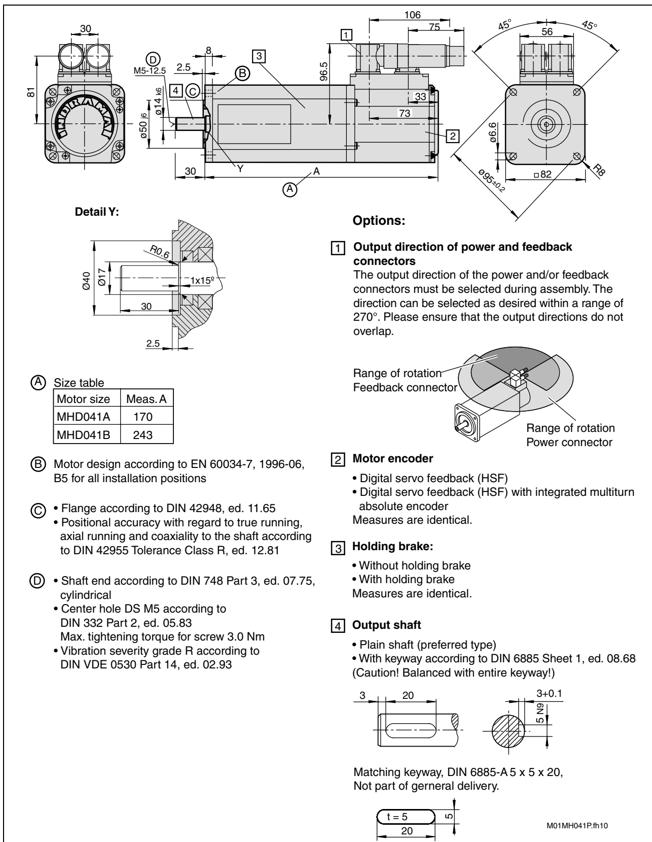
Fig. 6-8: Dimensional details of MHD041
