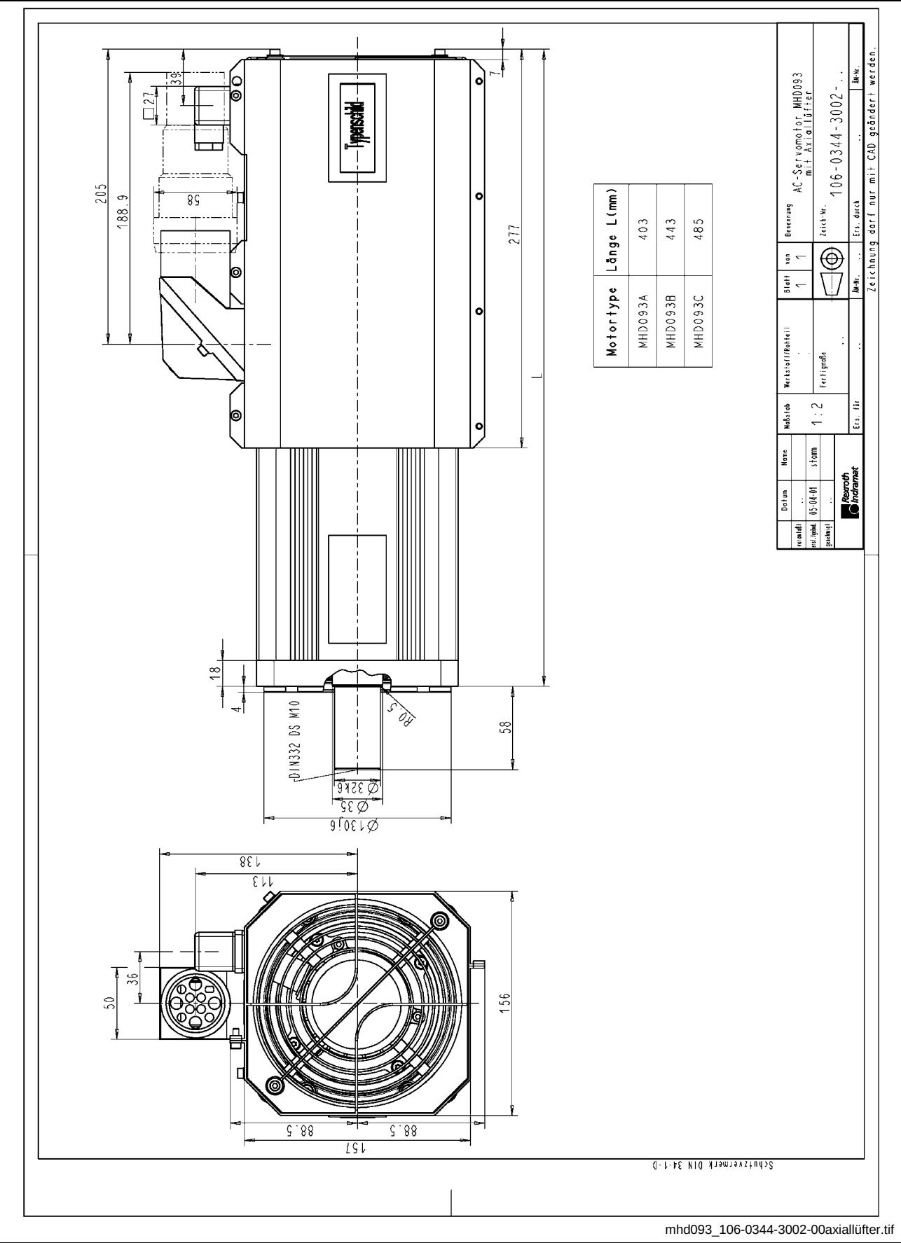
Fig. 9-20: Dimensional details of MHD093 with axial blower
