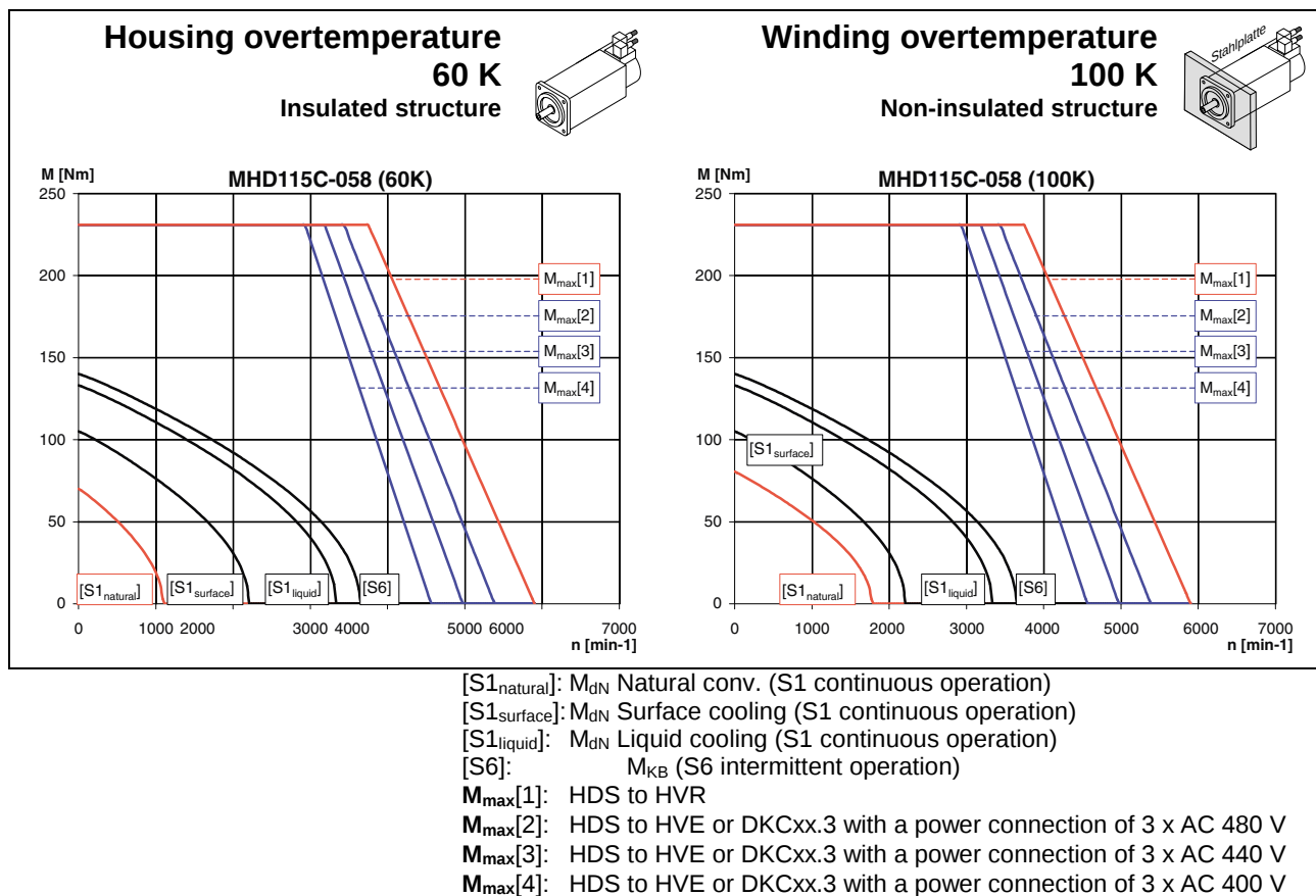
Fig. 12-14: Characteristic curves
