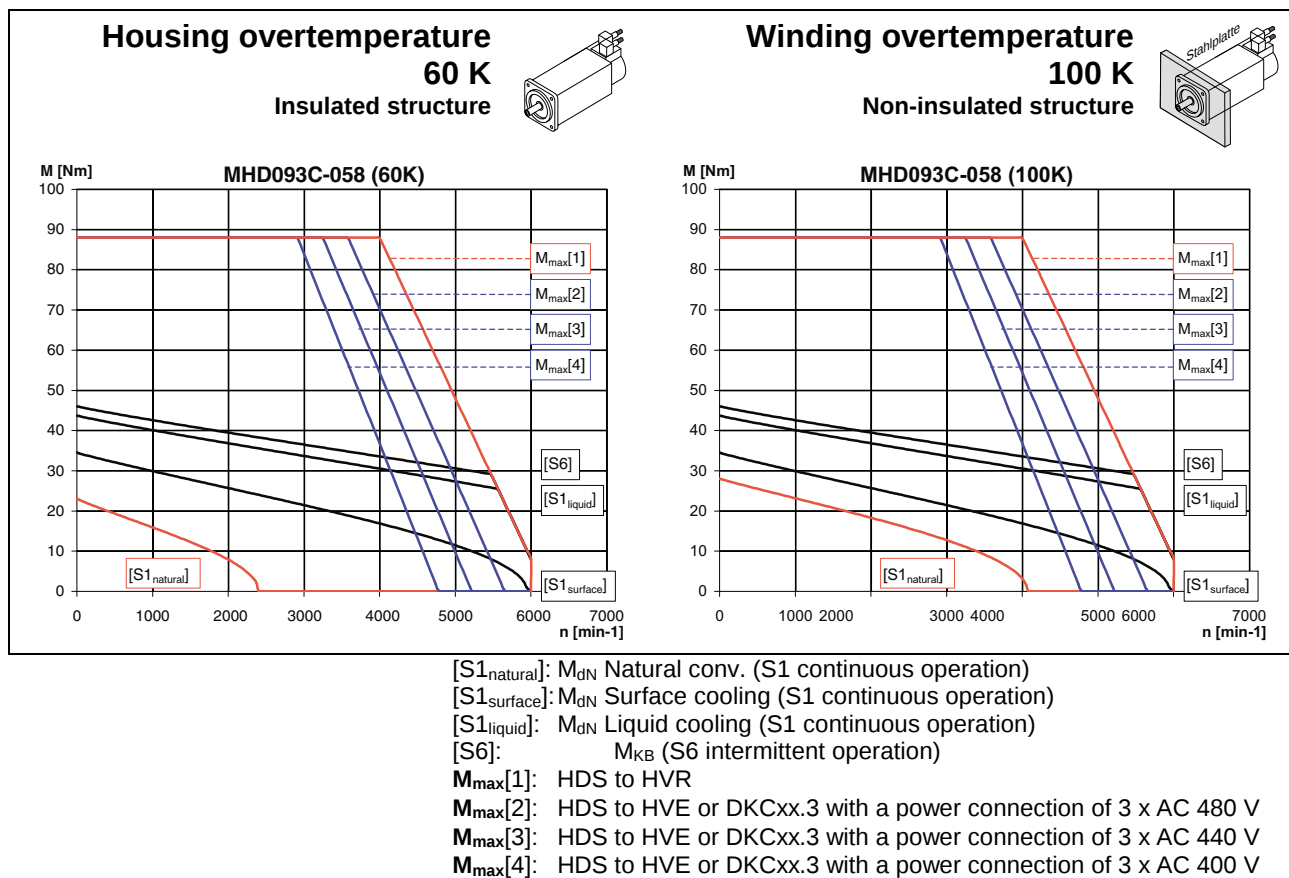
Fig. 9-14: Characteristic curves
