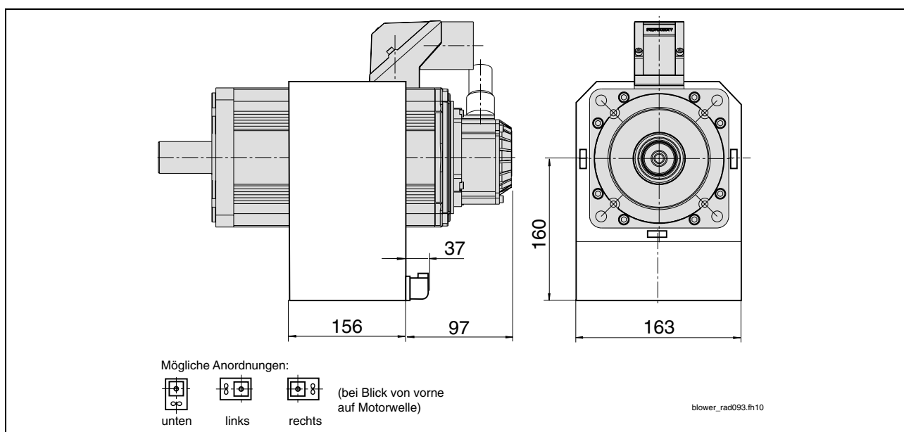
Fig. 9-19: Dimensional details of MHD093 with radial blower
