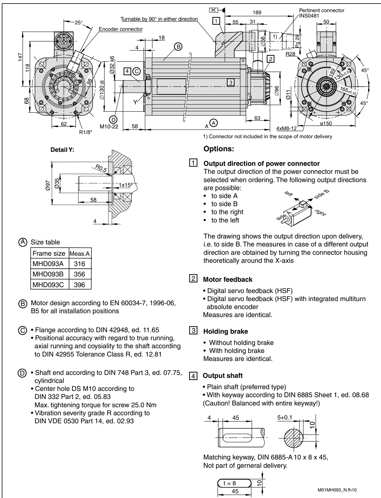
Fig. 9-21: Dimensional details of MHD093-....-N
