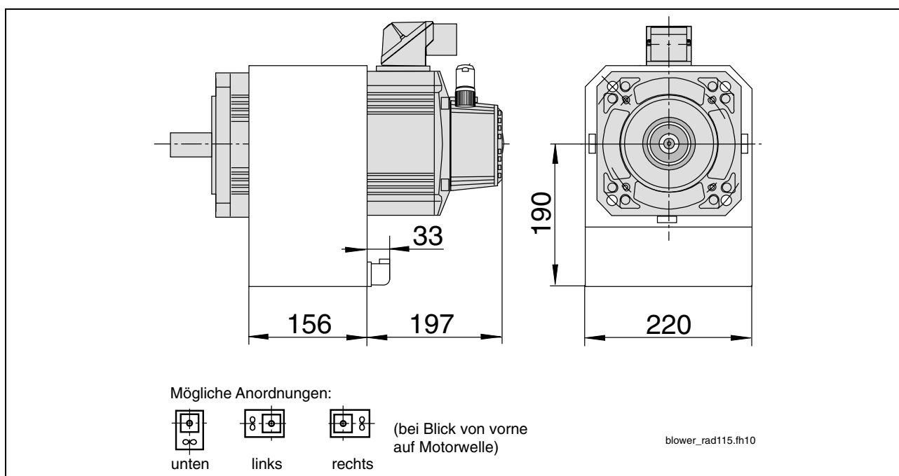
Fig. 12-20: Dimensional details about MHD115 with radial blower
