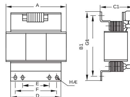
Lying version for wall mounting type DST.../L
