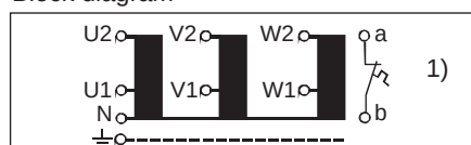
Block diagram
