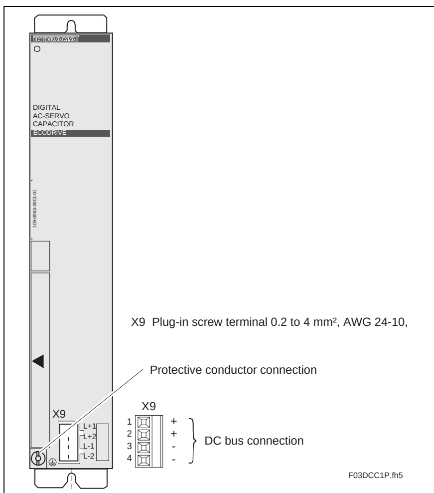
Fig. 6-7: Front view of the auxiliary capacitance module CZM01.1
