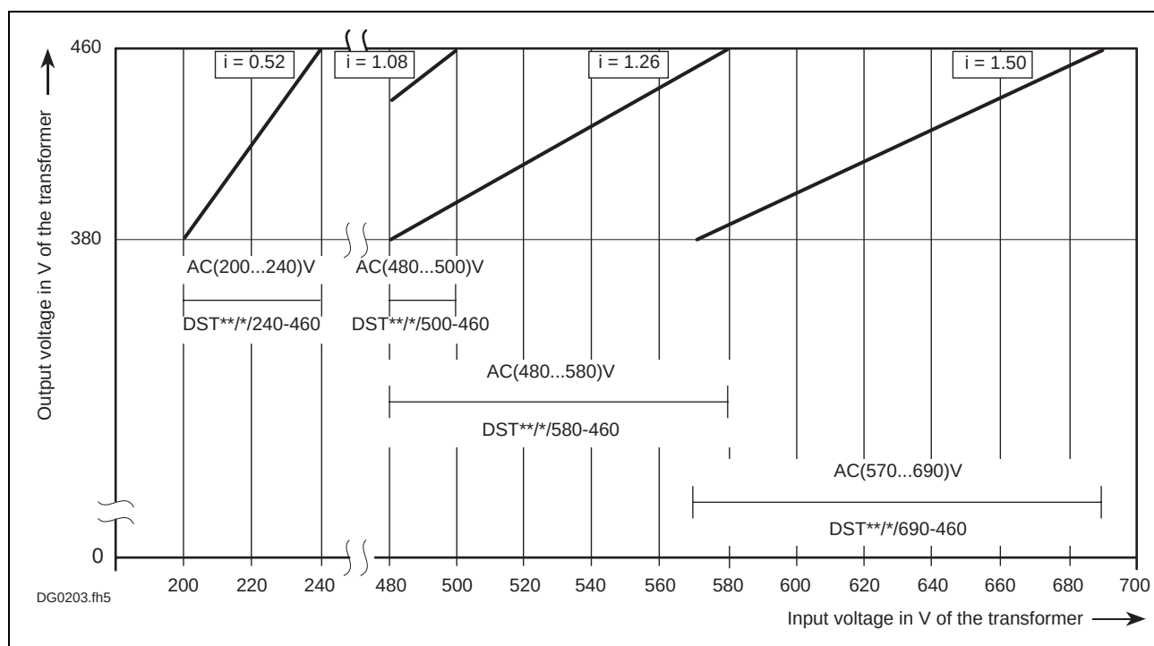
Fig. 9-1: Classification of three-phase autotransformers into rating groups
