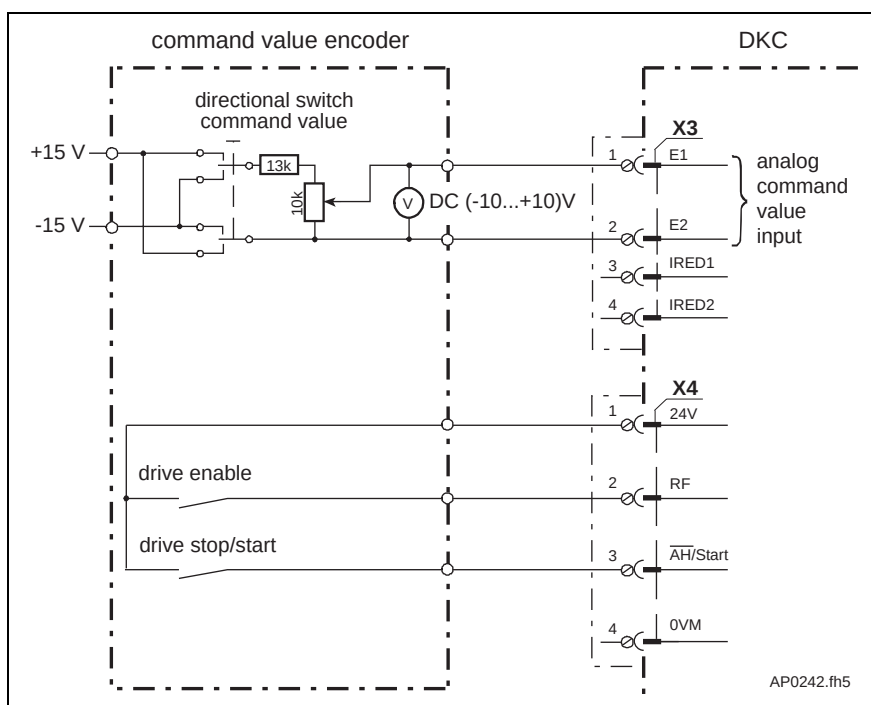
Fig. 12-1: Circuit proposal setpoint generator for connecting an analog interface
