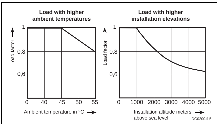
Fig. 4-8: Load utilization as a value dependent upon ambient temperature and installation altitude
