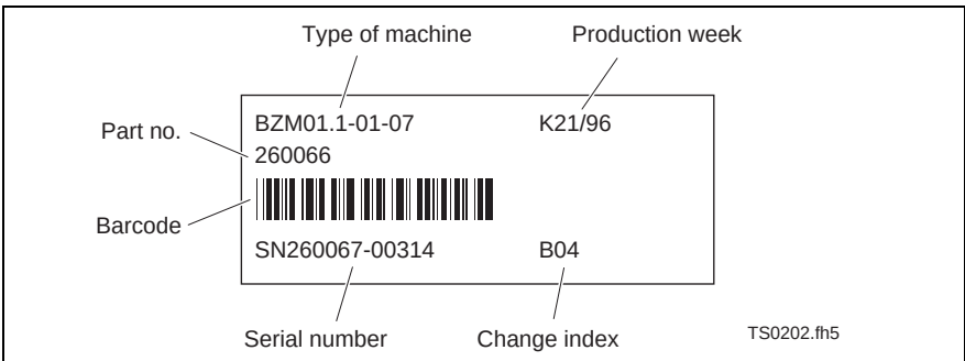
Fig. 5-9: Rating plate
