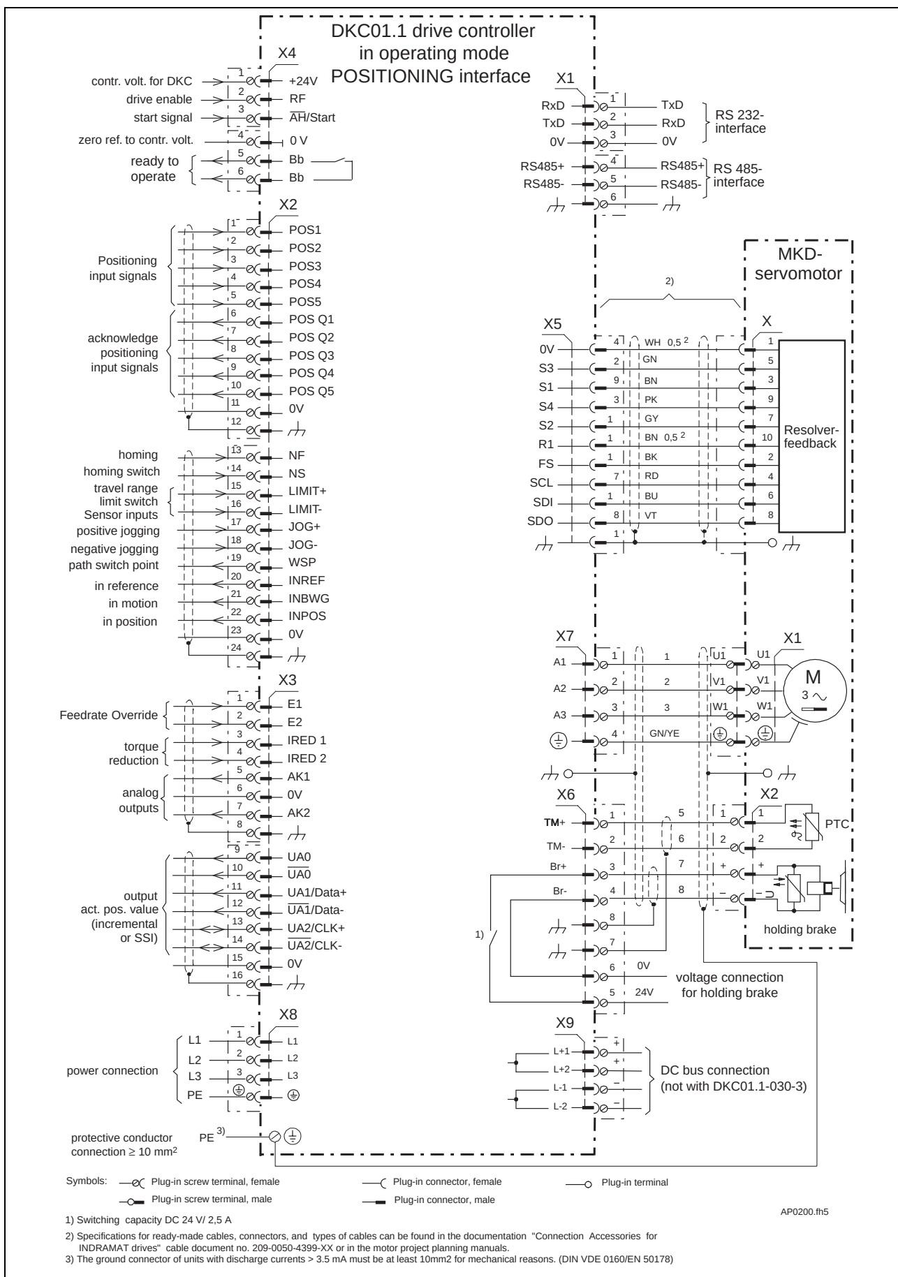
Fig. 4-15: DKC01.1 with POSITIONING interface
