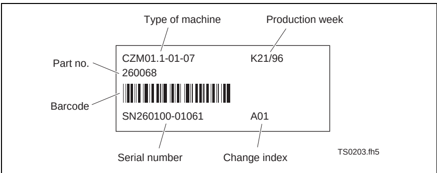
Fig. 6-10: Rating plate
