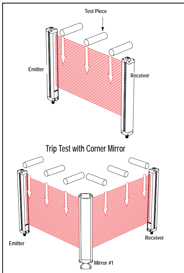
Figure 3-15. EZ-SCREEN trip test
