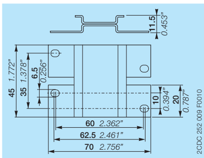
ADP.02 - Adapter for screw mounting
