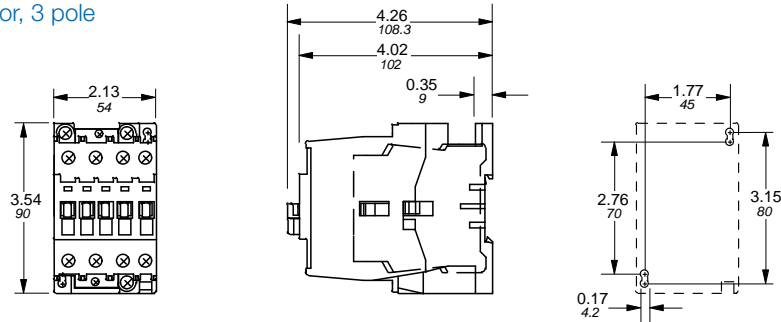
A/AE30 & A/AE40 + VM5 or VE5 – Mechanically interlocked contactor, 3 pole
