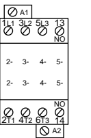
= AL9 – AL40-30-10 + CA5-01 + CA5-10
