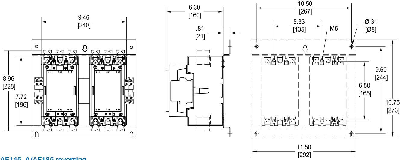
A/AF145, A/AF185 reversing
