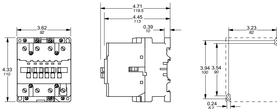
A/AE/AF45 – A/AE/AF75 — Contactor, 4 pole
