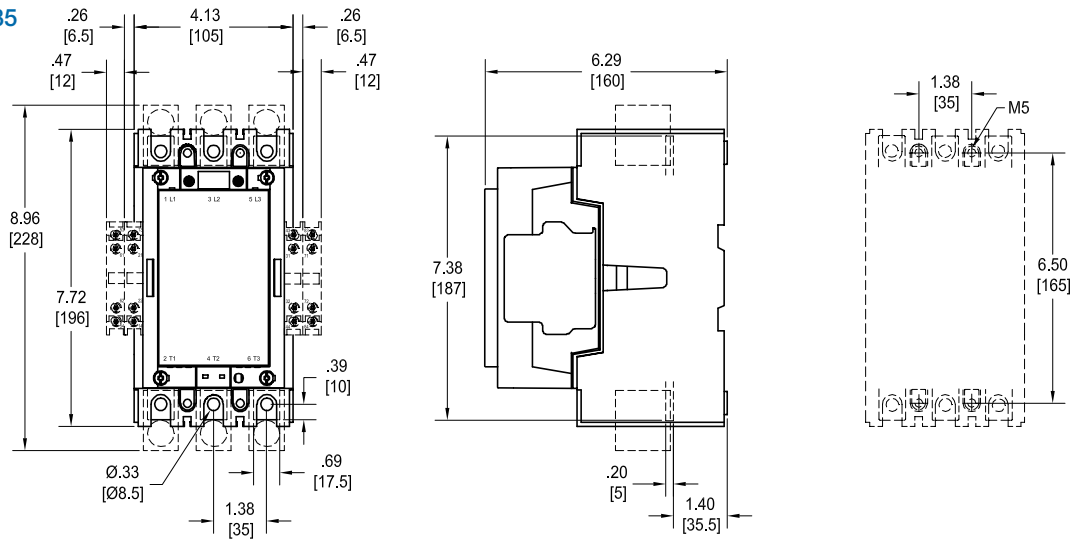
A/AF145, A/AF185 with mechanical interlock
