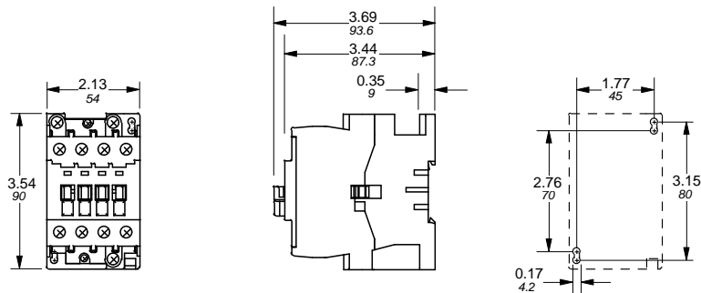
A/AE/AF45 – A/AE/AF75 — Contactor, 4 pole
