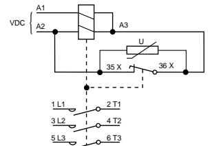
Coil wiring
