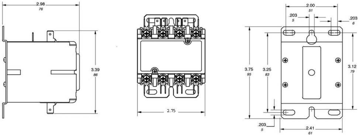
DP50 to DP60, 3 poles
