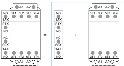
Combination 11 = CAL4-11 + AF09 ... AF38-40-00
