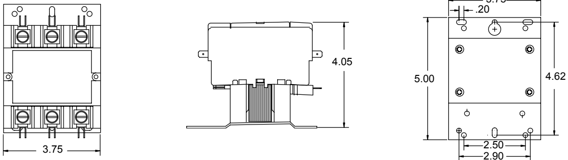
DP75 to DP90, 3 poles
