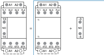
Combination 10 = AF09 ... AF38..-40-00 + CA4-10
