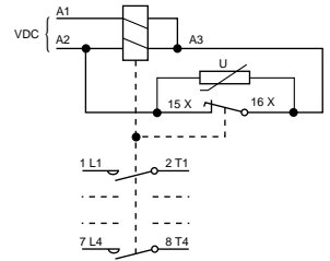
Coil wiring
