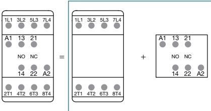
Combination 11 = AF09 ... AF38..-40-00 + CAT4-11E
