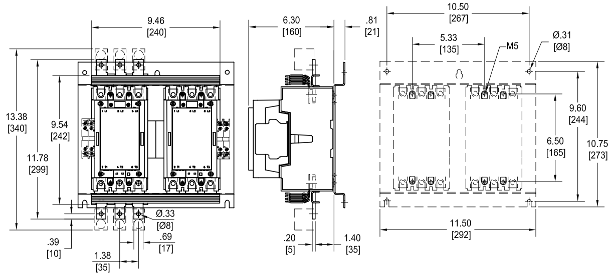
A/AF145, A/AF185 reversing
