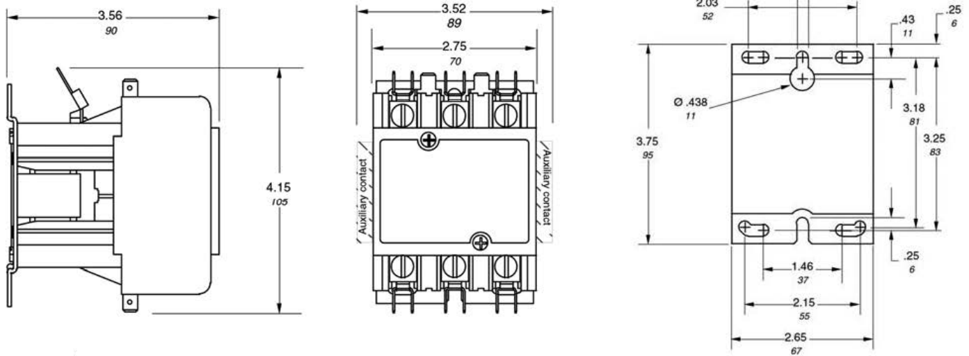
DP75 to DP90, 3 poles
