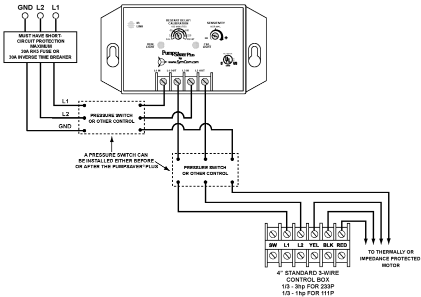
FIGURE 2: Standard Control Box Wiring Diagram
