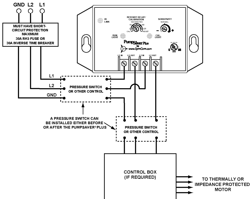
FIGURE 1: Typical Wiring Diagram
